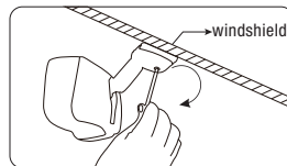
With an Allen key, fix rear view mirror Torque is about 0.8-1.3 Nm
